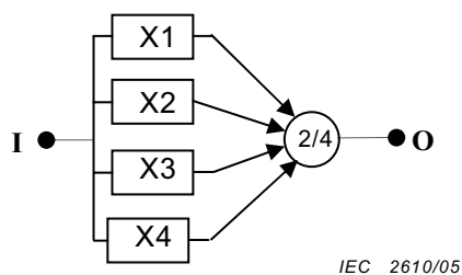
Figure 7 – Redondance 2/4
