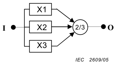
Figure 6 – Redondance 2/3
