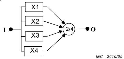
Figure 7 – 2/4 redundancy
