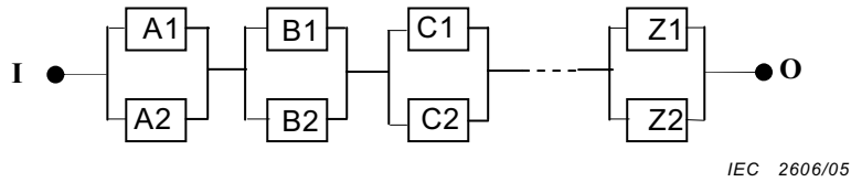
Figure 3 – Series duplicated (or parallel) reliability block diagram
