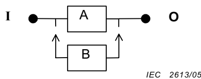
Figure 10 – Standby redundancy
