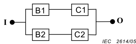
Figure 11 – Representation of Figure 8 when item A has failed
