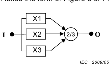
Figure 6 – 2/3 redundancy
