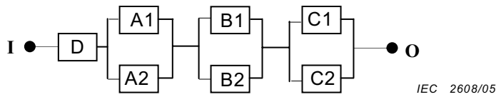
Figure 5 – Another type of mixed redundancy reliability block diagram
